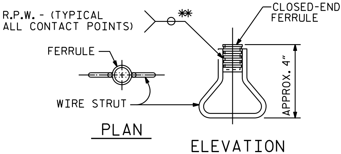
CONCRETE INSERT
